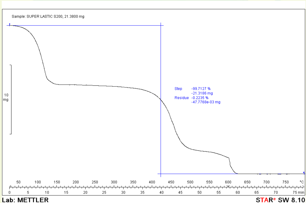
Figure B.1. TGA Thermogram of 'SUPER LASTIC S200' Sample
